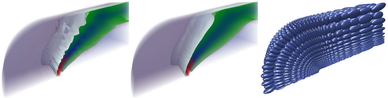
Fig. 6. The irregular blunt fin data set rendered using a standard tetrahedral rendering scheme ( left ), the proposed MLS technique with adaptive preintegration ( middle ), and the anisotropic weights used in the MLS reconstruction ( right ).
